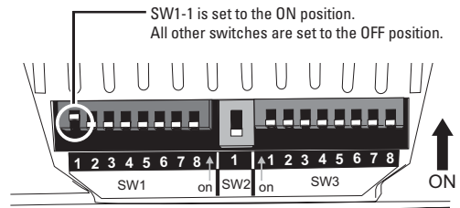
Figure 1. Default Switch Settings
