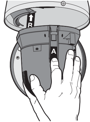
Figure 2. Dome Drive Installation
